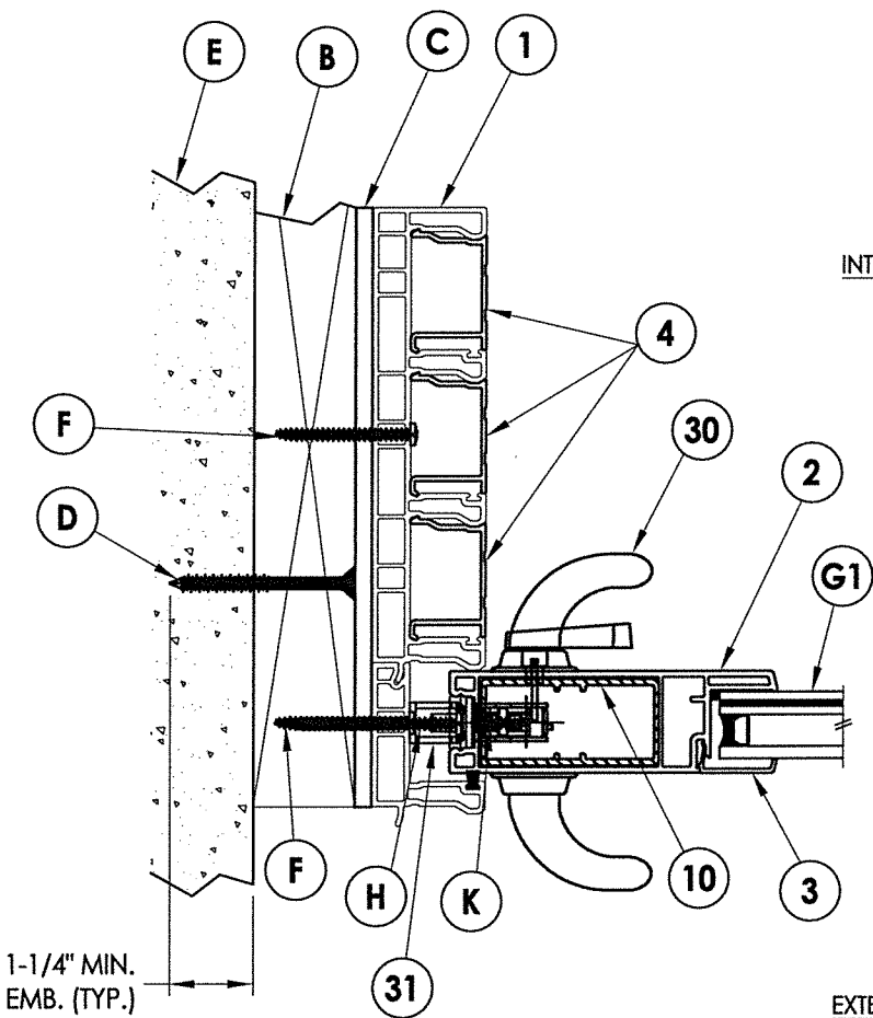
1 3 HORIZONTAL CROSS SECTION 2X Buck Construction
